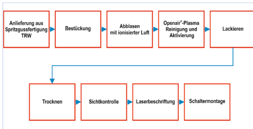
Flow diagram of switch production including the painting process.
